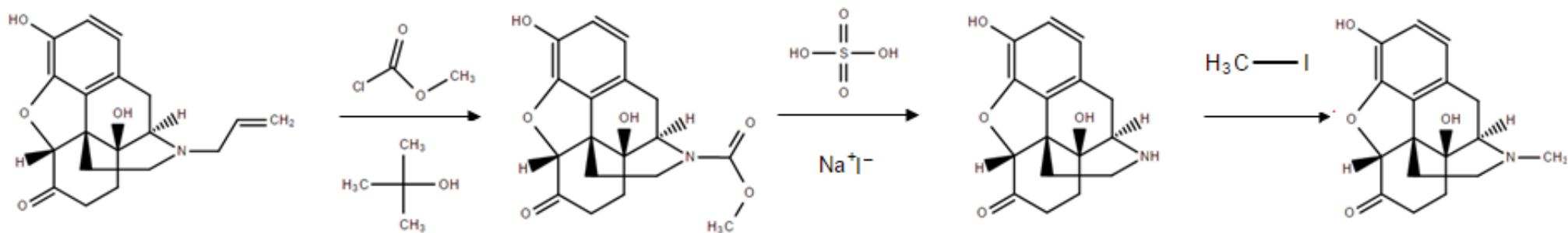
Reaction Scheme for Conversion of Naloxone to Oxymorphone
